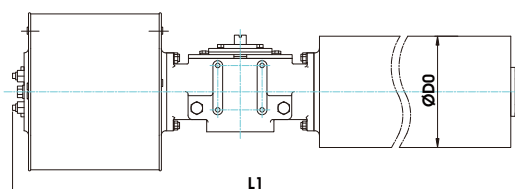
Single Acting
