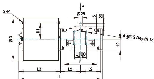
Double Acting
